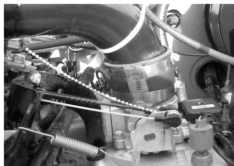
Speed control to throttle attachment (side view)
